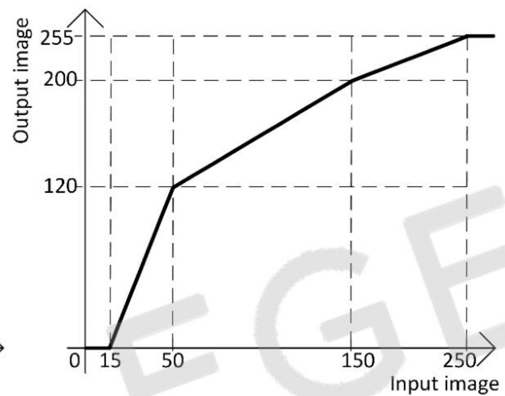
Piece-wise linear contrast stretch (2)
