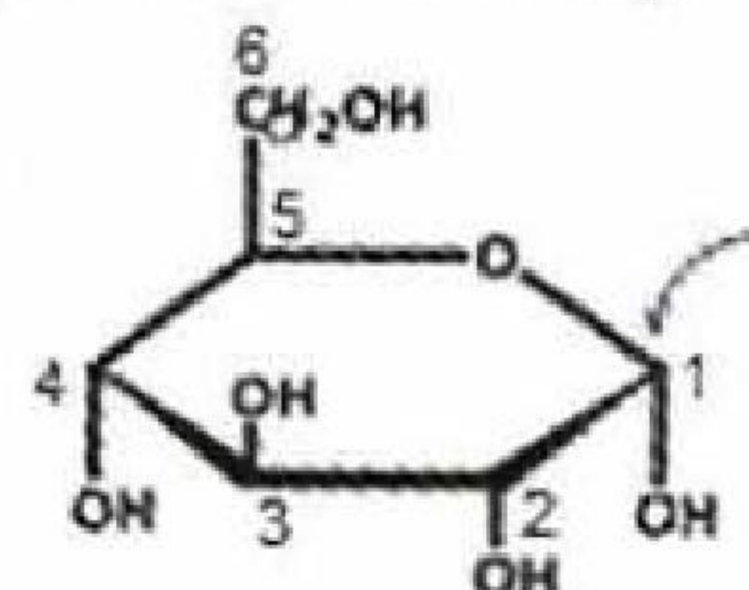
\alpha -D-glucopyranose
