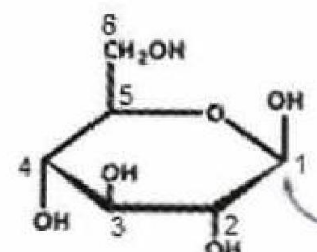
\beta -D-glucopyranose
