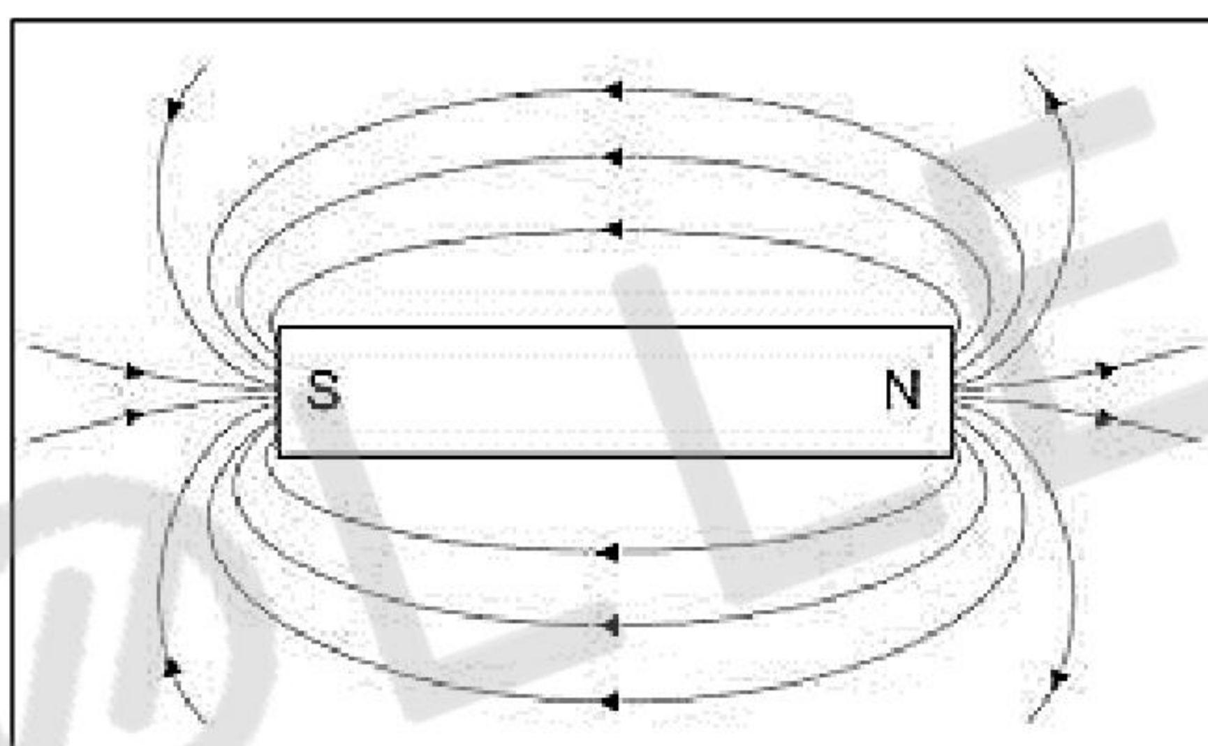
Magnetic field lines of a bar magnet
