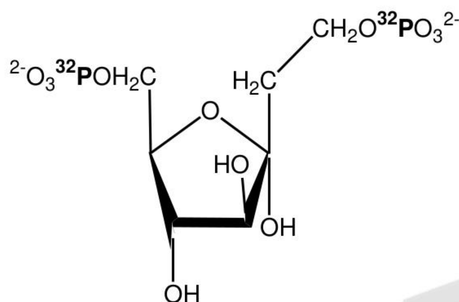
Fructose 1,6-bisphosphate
