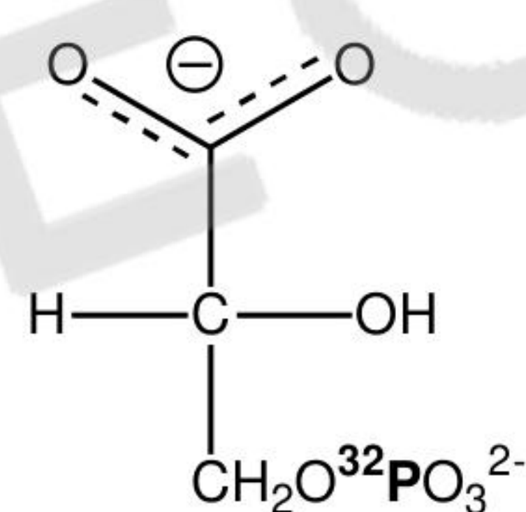
3-Phosphoglycerate
