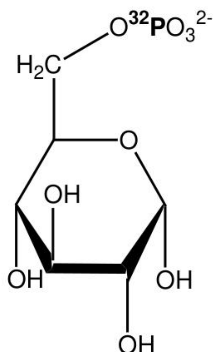
Glucose 6-phosphate
