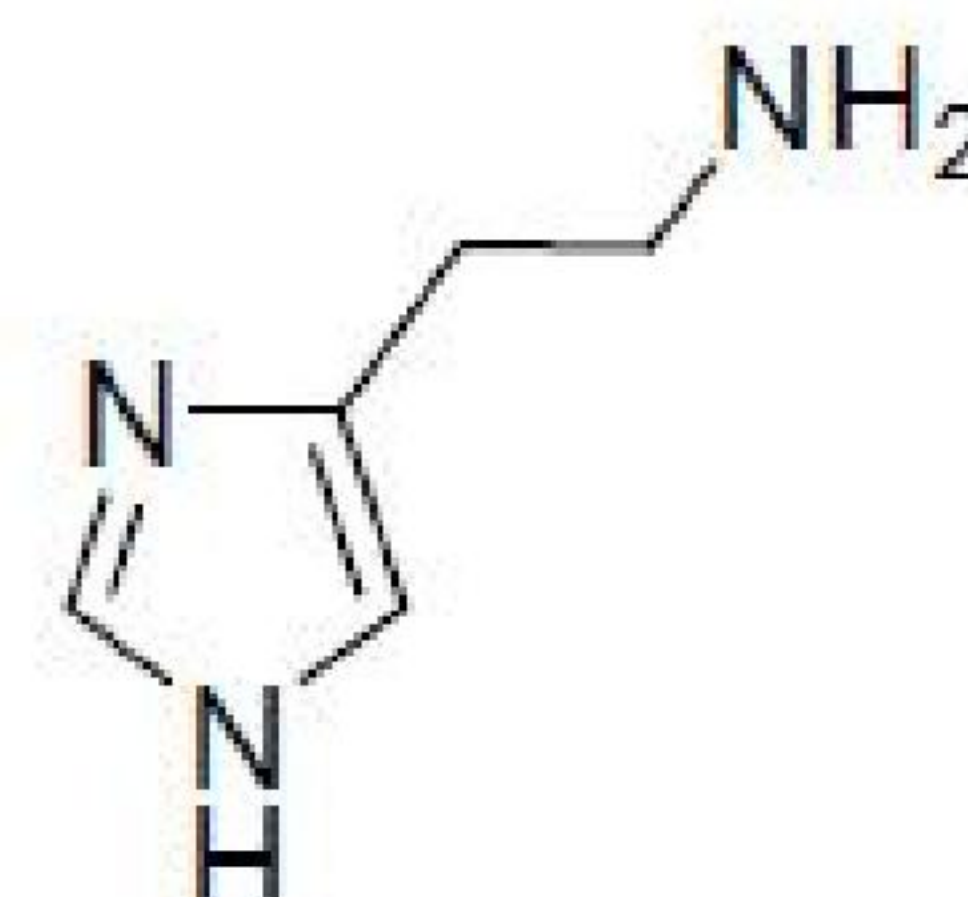
Histamine
