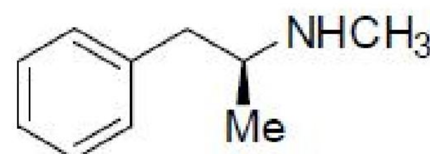
Methamphetamine
